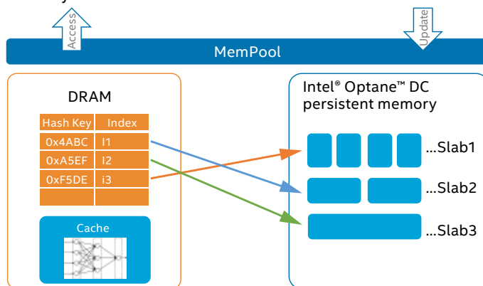
Fig. 3 Heterogeneous storage system built on Intel® Optane™ DC persistent memory
