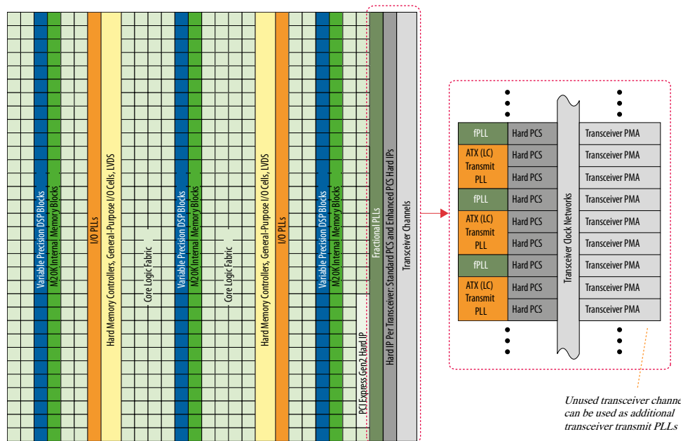
Figure 2. Cyclone 10 GX FPGA Architecture Block Diagram
