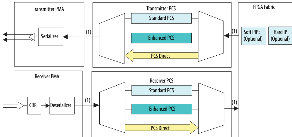
Figure 4. GX Transceiver Channel in Full Duplex Mode
