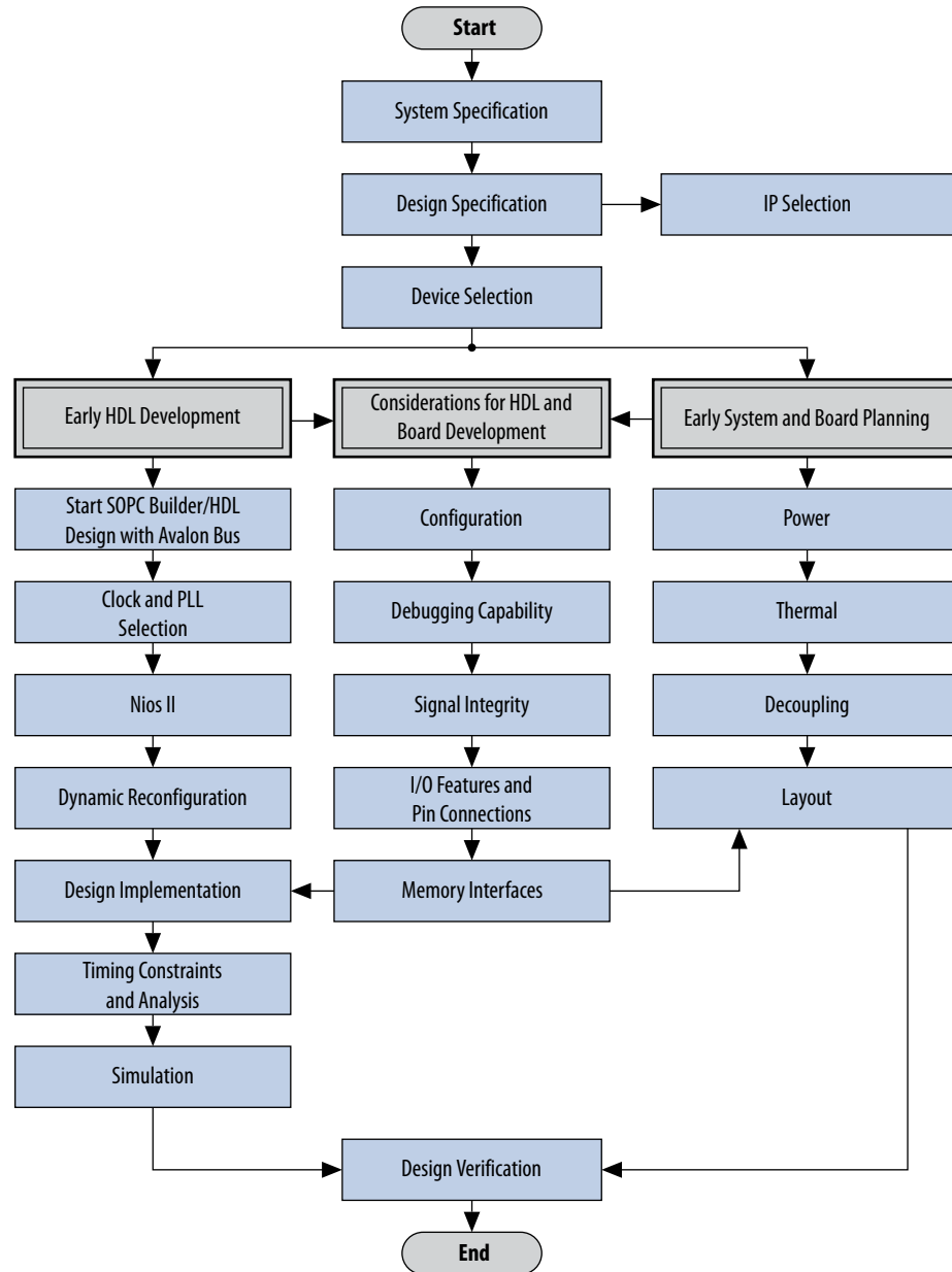
Figure 1. Cyclone 10 GX Device Design Flow
