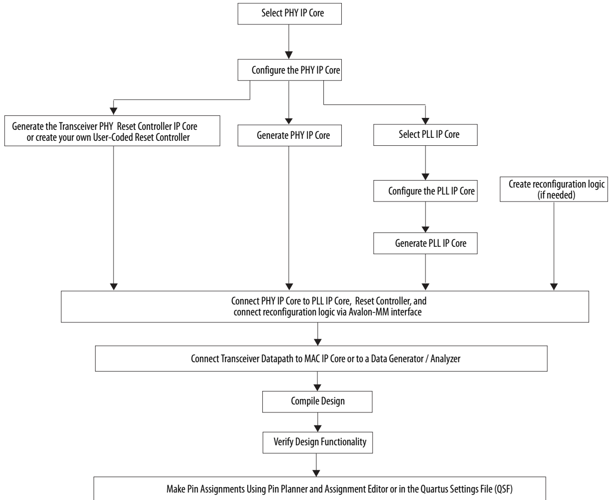
Figure 5. Transceiver Design Flow
